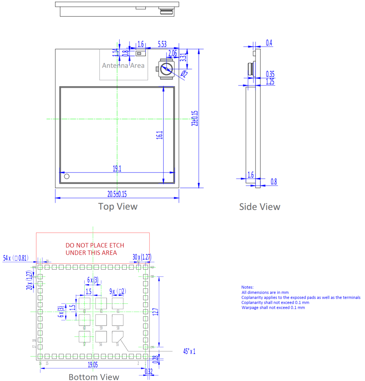
Figure 5-1: Mechanical Drawing
